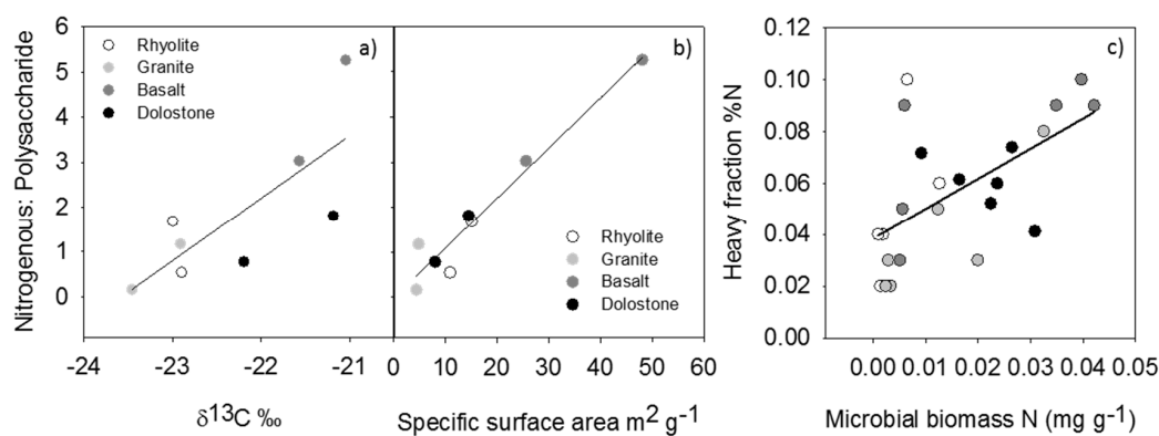
Figure 3. (a) Heavy fraction \delta^{13}\text{C} abundance vs. nitrogenous: polysaccharide, r^2 = 0.60 , p = 0.0241 ; (b) heavy fraction specific surface area vs. nitrogenous: polysaccharide, r^2 = 0.95 , p < 0.0001 ; (c) heavy fraction %N vs. microbial biomass N, r^2 = 0.39 , p = 0.0015 .
